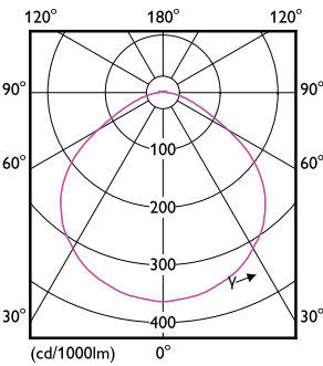
Light Distribution Diagram - TForce HB 140W E40 840 WB GM
