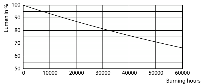
Lumen Maintenance Diagram - TForce HB 140W E40 840 WB GM
